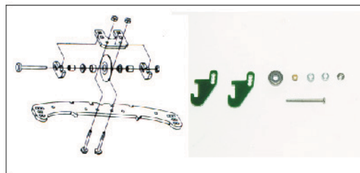
■ 910012 Fiberglass 360° Rotation Fixture Set (Front)
