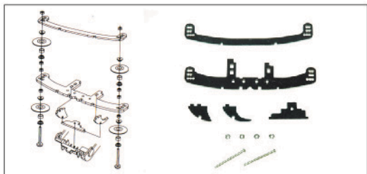
■ 910009 Fiberglass Stabilizer Bumper (Front)
